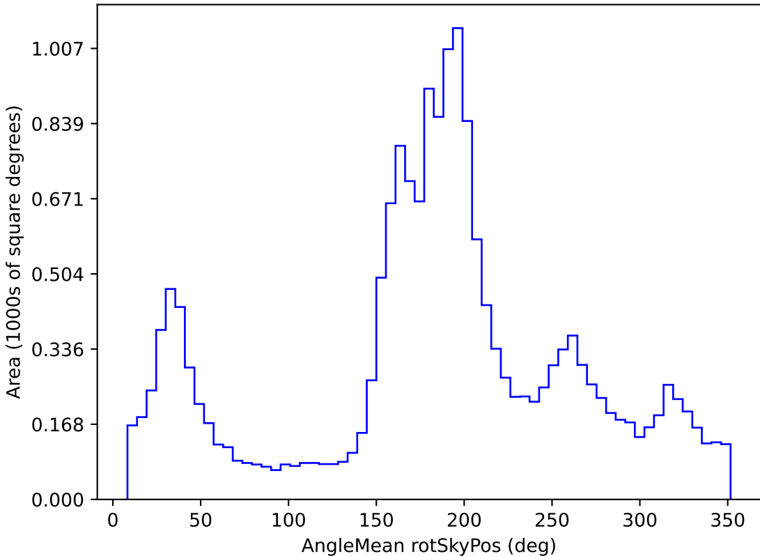
weather_cloudso31v3.4_10yrs WFD u band: AngleMean rotSkyPos
