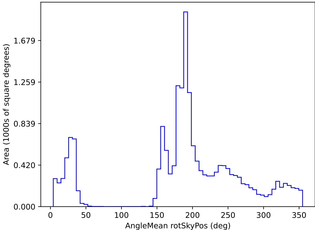
weather_cloudso31v3.4_10yrs WFD all bands: AngleMean rotSkyPos
