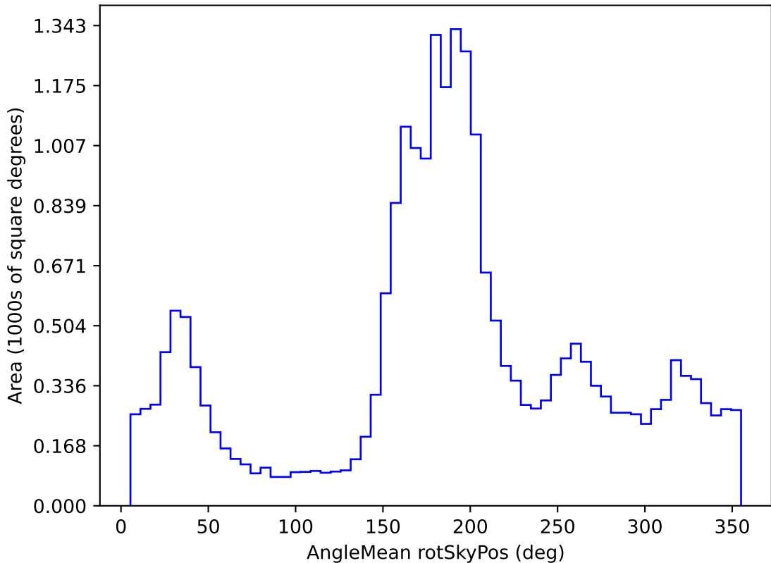
weather_cloudso31v3.4_10yrs All sky u band: AngleMean rotSkyPos
