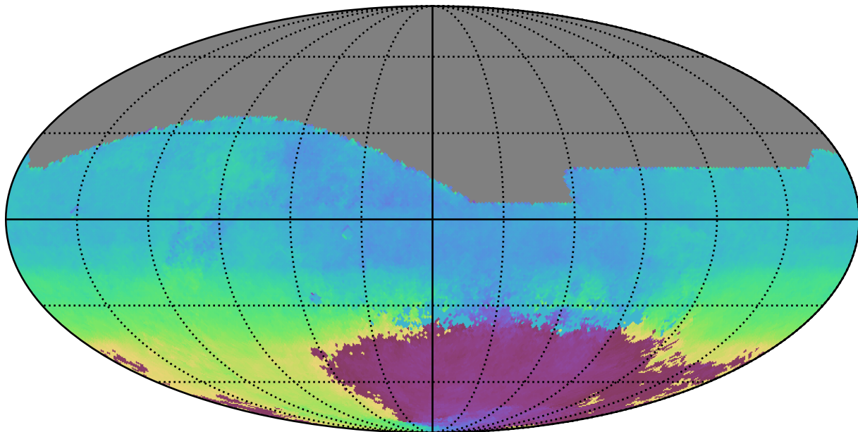
weather_cloudso31v3.4_10yrs All sky r band: AngleMean rotSkyPos
