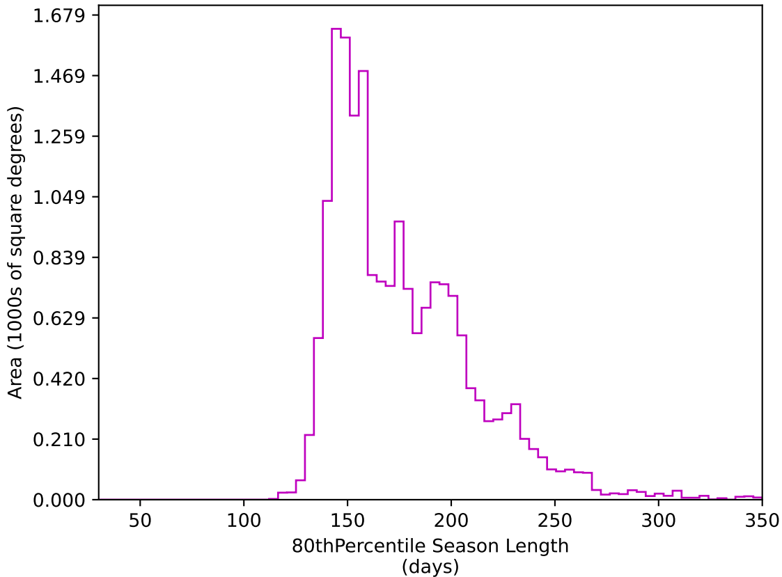
weather_cloudso31v3.4_10yrs WFD z band: 80thPercentile Season Length
