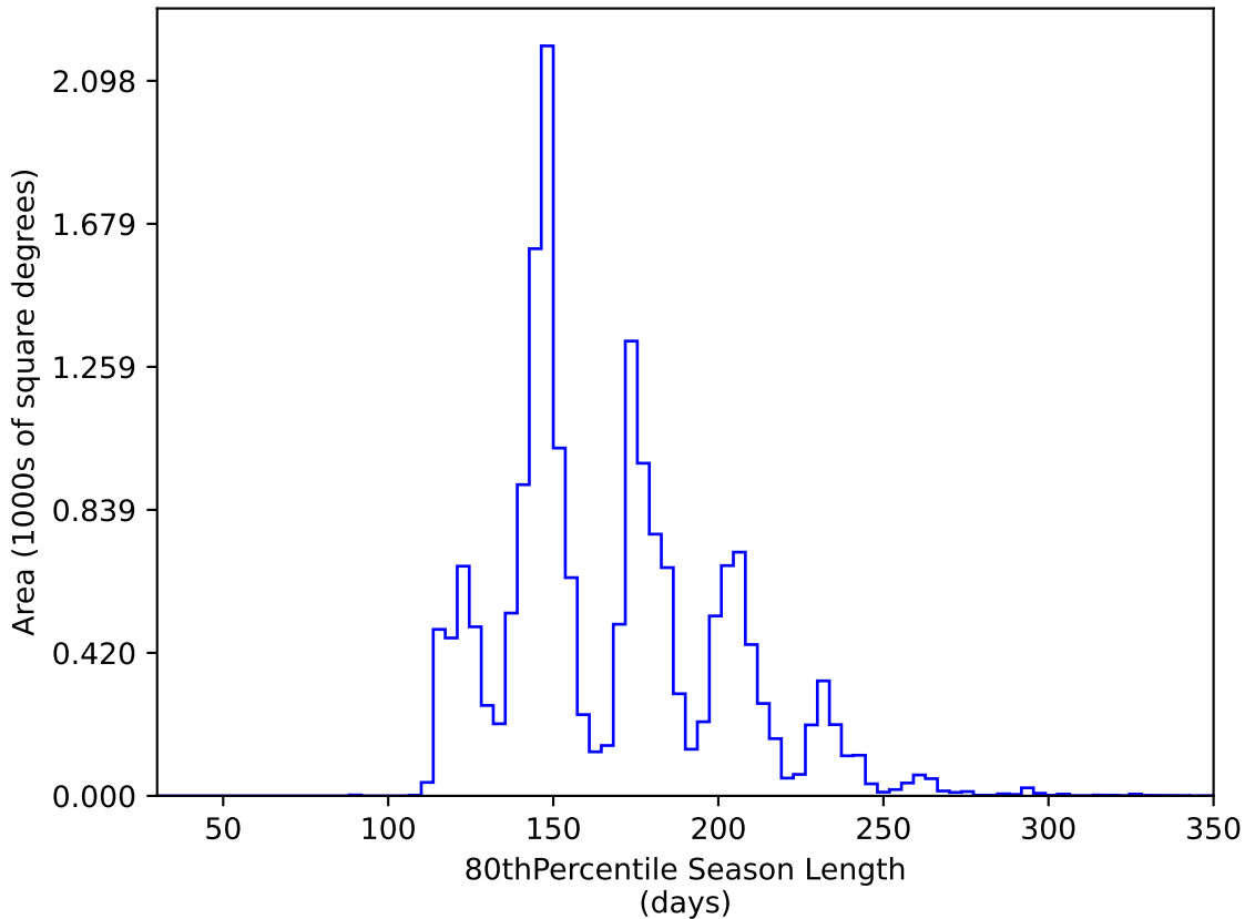
weather_cloudso31v3.4_10yrs WFD y band: 80thPercentile Season Length
