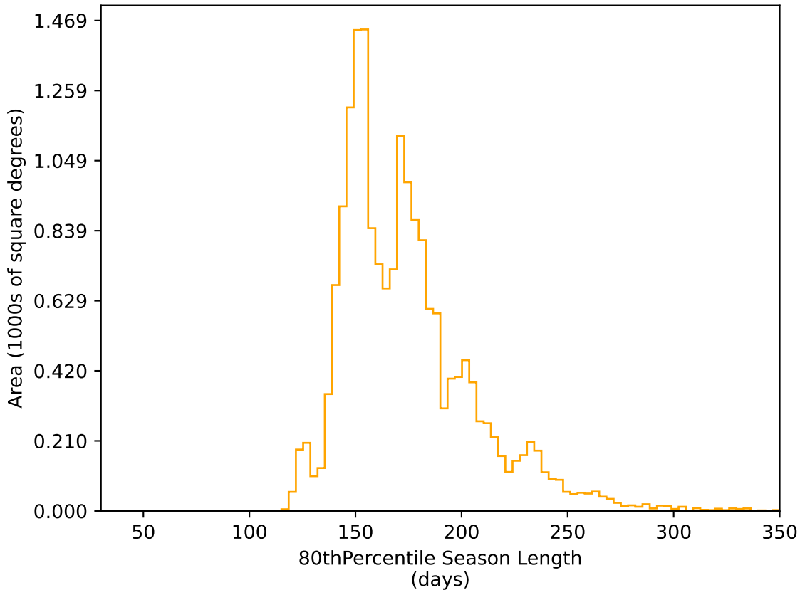
weather_cloudso31v3.4_10yrs WFD r band: 80thPercentile Season Length
