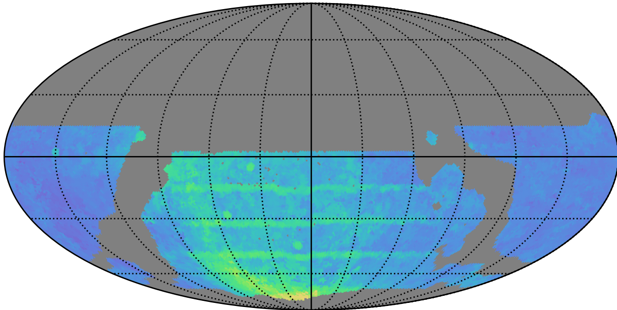
weather_cloudso31v3.4_10yrs WFD i band: 80thPercentile Season Length
