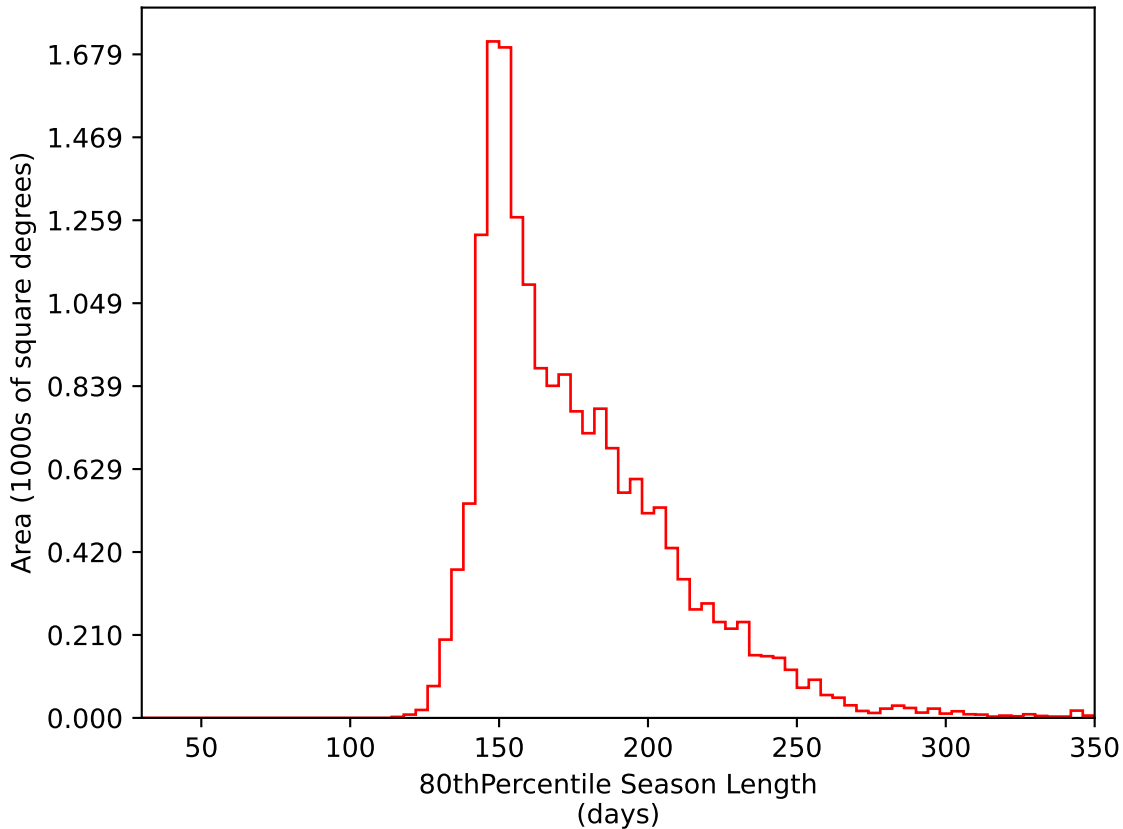
weather_cloudso31v3.4_10yrs WFD i band: 80thPercentile Season Length
