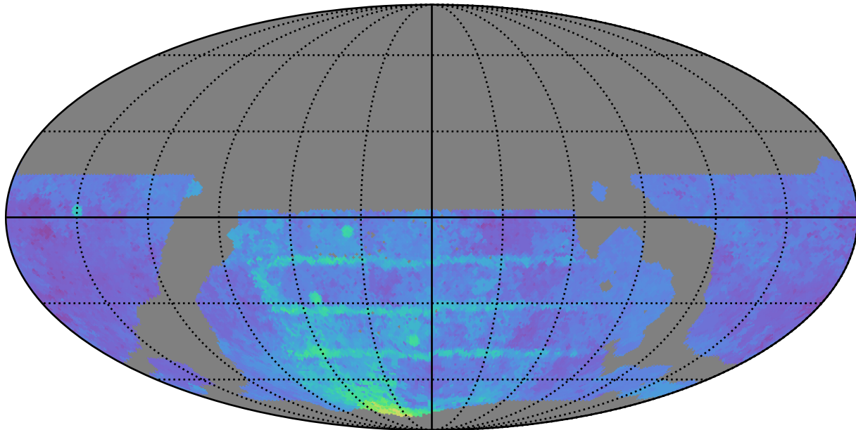
weather_cloudso31v3.4_10yrs WFD g band: 80thPercentile Season Length
