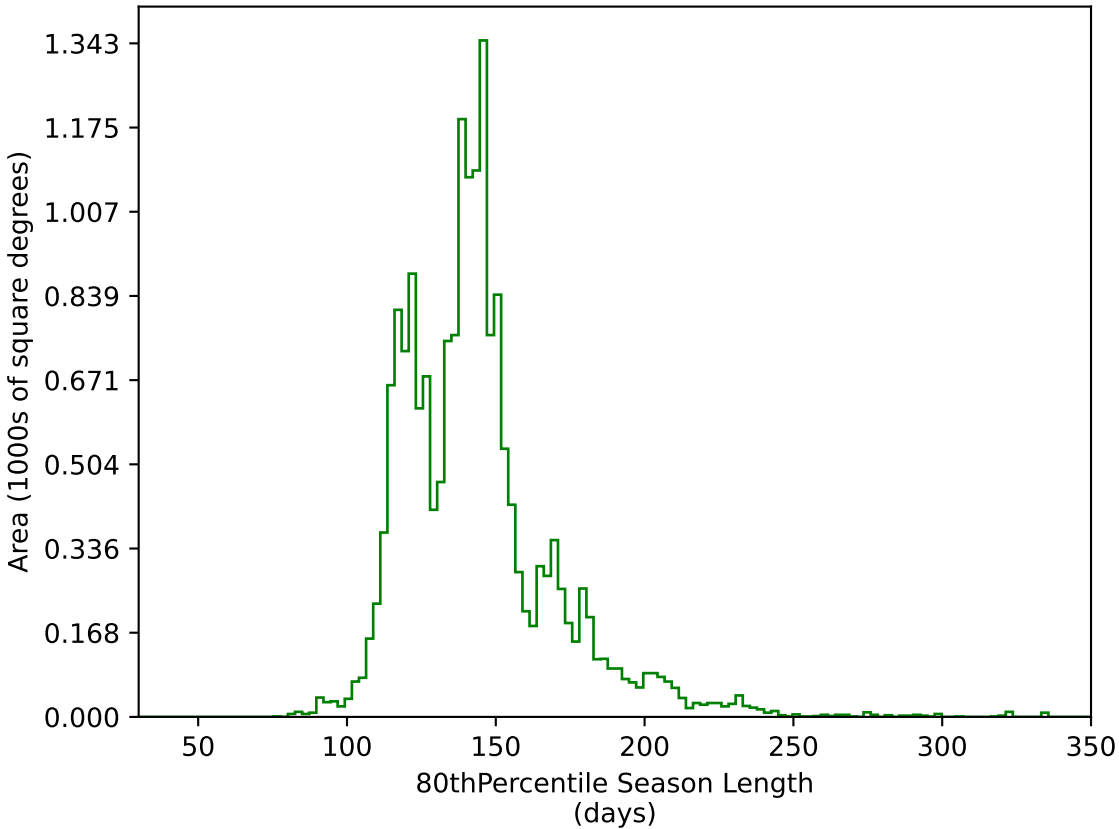
weather_cloudso31v3.4_10yrs WFD g band: 80thPercentile Season Length
