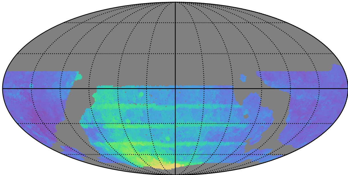
weather_cloudso31v3.4_10yrs WFD all bands: 80thPercentile Season Length
