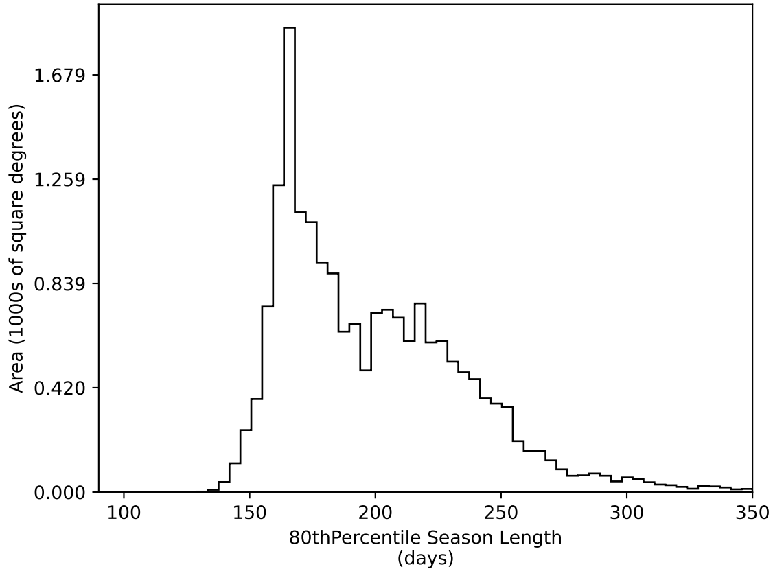
weather_cloudso31v3.4_10yrs WFD all bands: 80thPercentile Season Length
