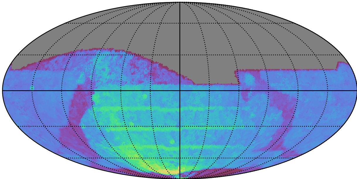
weather_cloudso31v3.4_10yrs All sky z band: 80thPercentile Season Length
