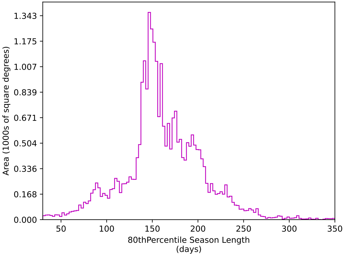
weather_cloudso31v3.4_10yrs All sky z band: 80thPercentile Season Length
