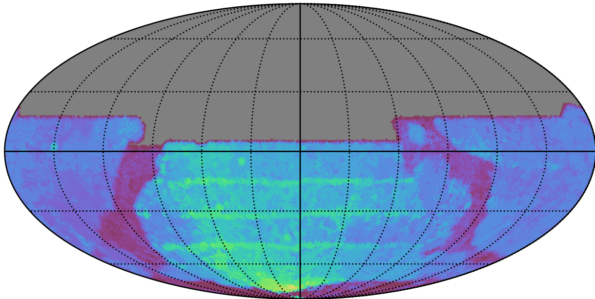
weather_cloudso31v3.4_10yrs All sky y band: 80thPercentile Season Length
