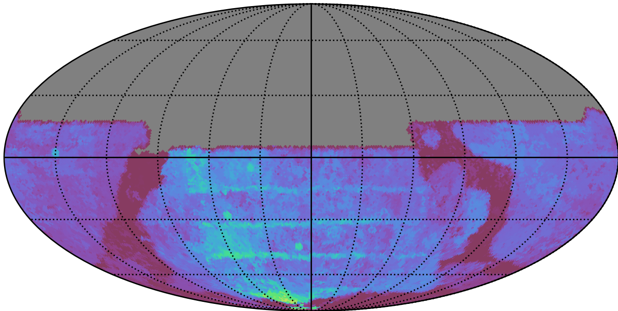
weather_cloudso31v3.4_10yrs All sky u band: 80thPercentile Season Length
