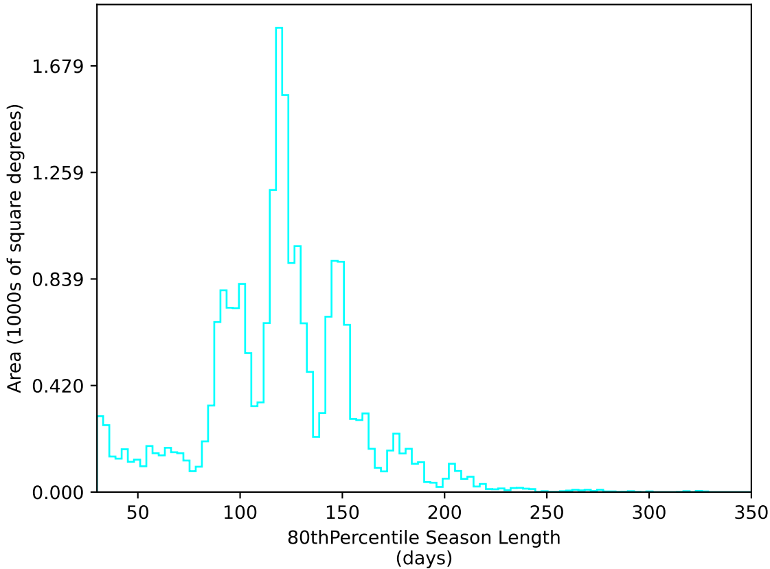
weather_cloudso31v3.4_10yrs All sky u band: 80thPercentile Season Length
