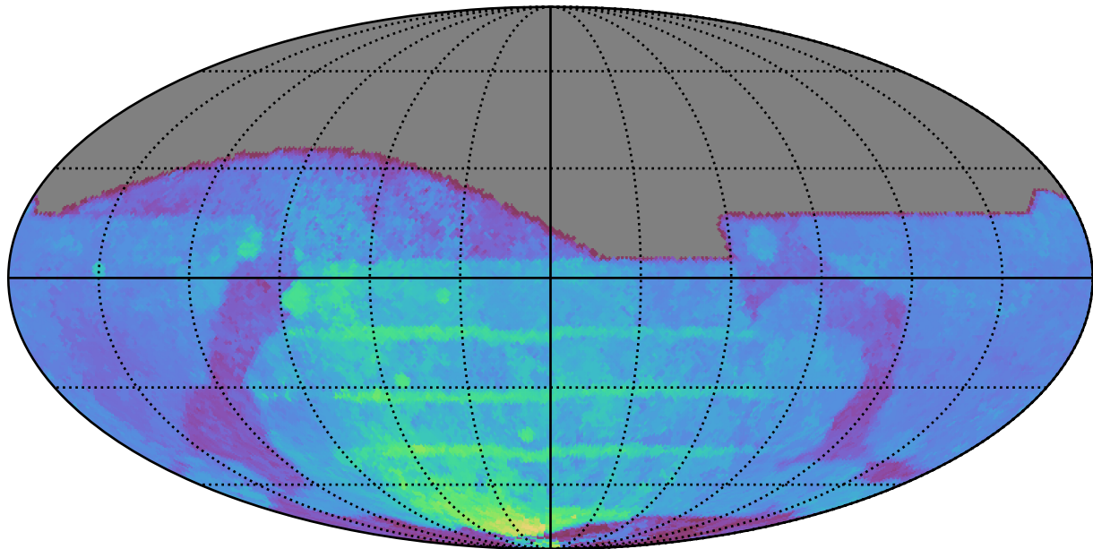
weather_cloudso31v3.4_10yrs All sky r band: 80thPercentile Season Length
