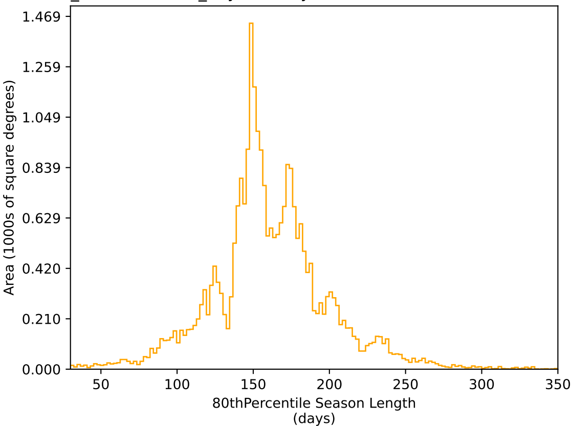
weather_cloudso31v3.4_10yrs All sky r band: 80thPercentile Season Length
