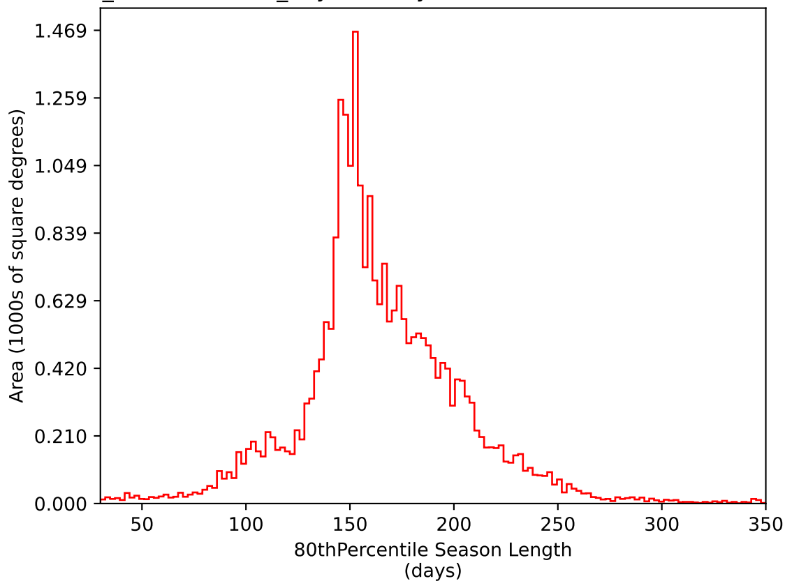
weather_cloudso31v3.4_10yrs All sky i band: 80thPercentile Season Length
