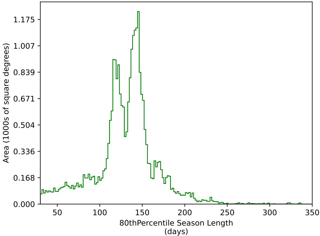
weather_cloudso31v3.4_10yrs All sky g band: 80thPercentile Season Length
