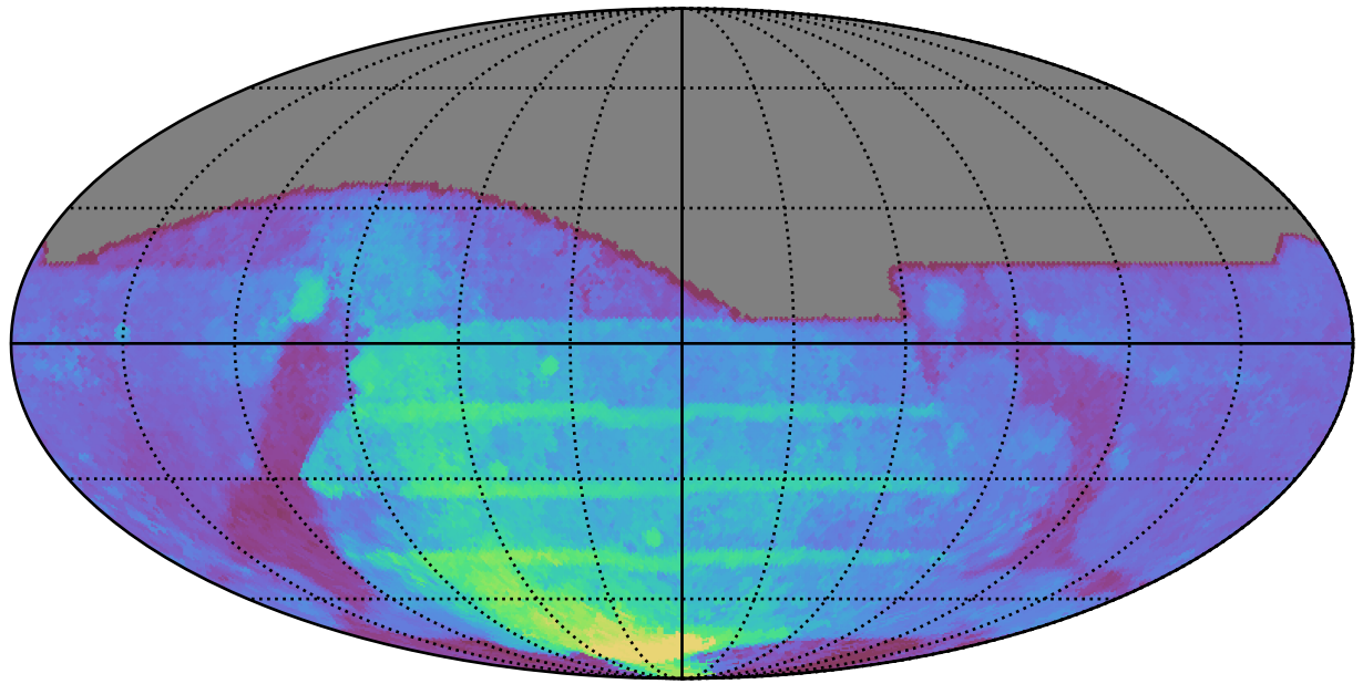
weather_cloudso31v3.4_10yrs All sky all bands: 80thPercentile Season Length
