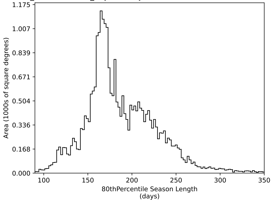
weather_cloudso31v3.4_10yrs All sky all bands: 80thPercentile Season Length
