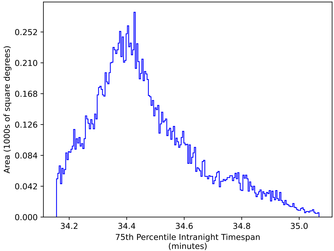
weather_cloudso31v3.4_10yrs WFD zy bands: 75th Percentile Intranight Timespan
