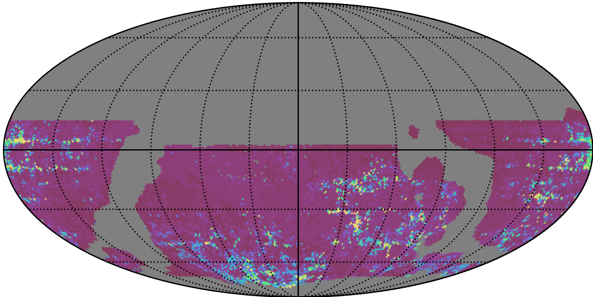
weather_cloudso31v3.4_10yrs WFD z band: 75th Percentile Intranight Timespan
