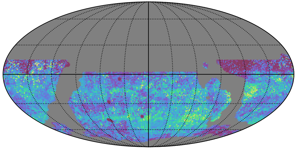
weather_cloudso31v3.4_10yrs WFD y band: 75th Percentile Intranight Timespan
