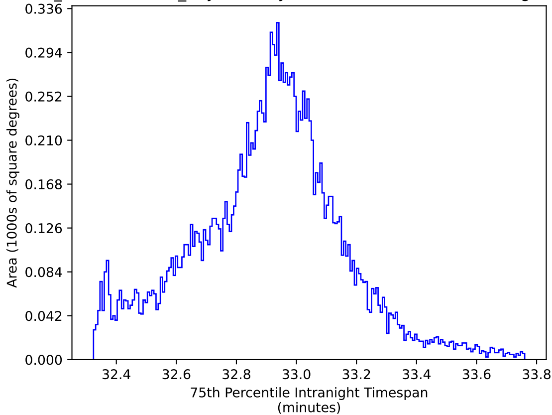
weather_cloudso31v3.4_10yrs WFD y band: 75th Percentile Intranight Timespan
