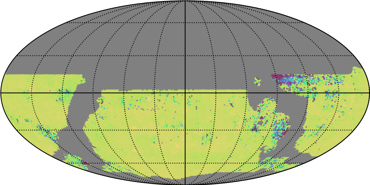
weather_cloudso31v3.4_10yrs WFD ug bands: 75th Percentile Intranight Timespan
