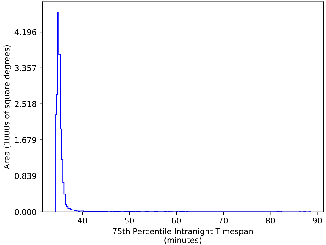
weather_cloudso31v3.4_10yrs WFD ri bands: 75th Percentile Intranight Timespan
