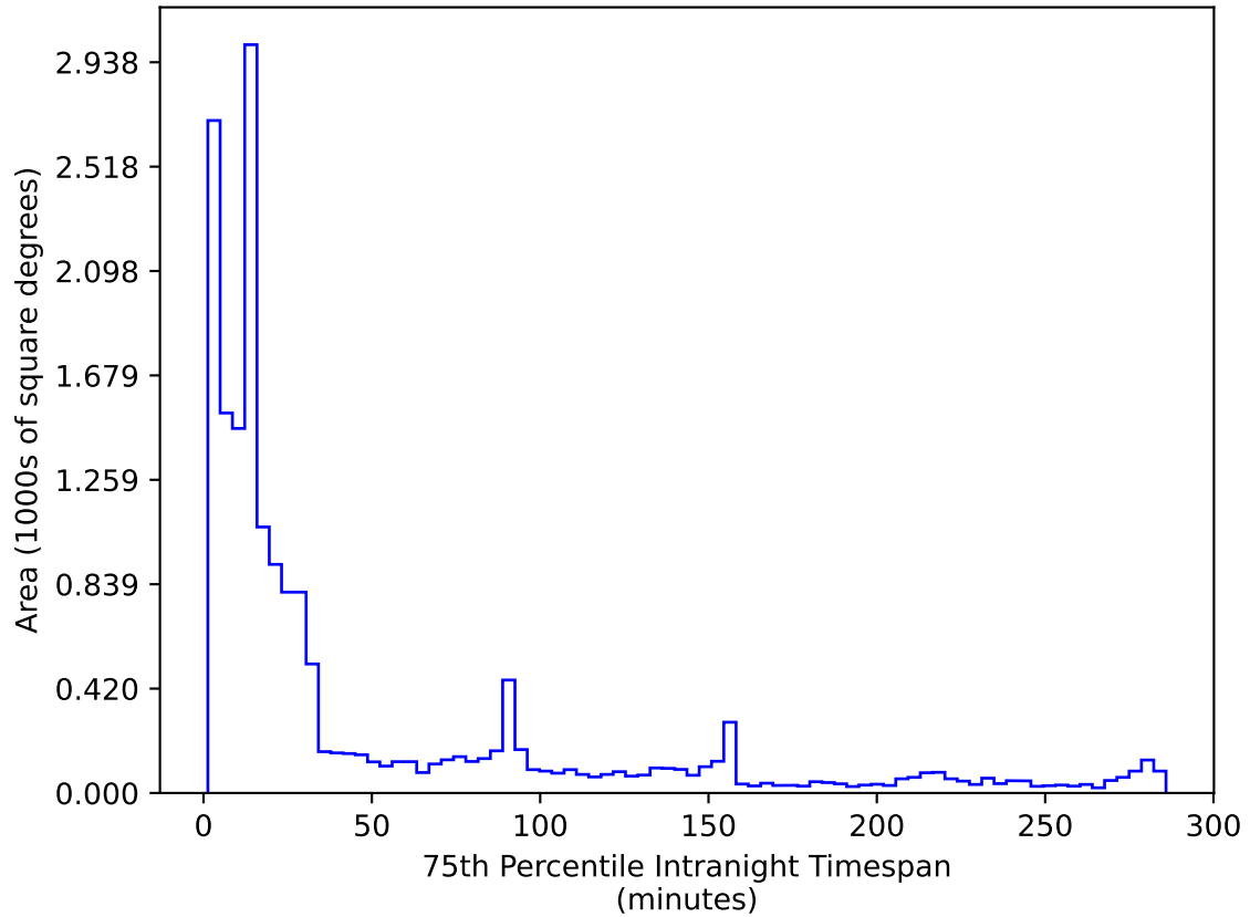
weather_cloudso31v3.4_10yrs WFD r band: 75th Percentile Intranight Timespan
