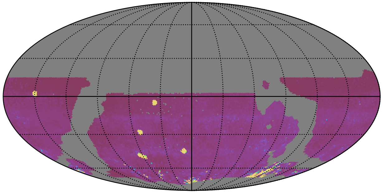
weather_cloudso31v3.4_10yrs WFD iz bands: 75th Percentile Intranight Timespan
