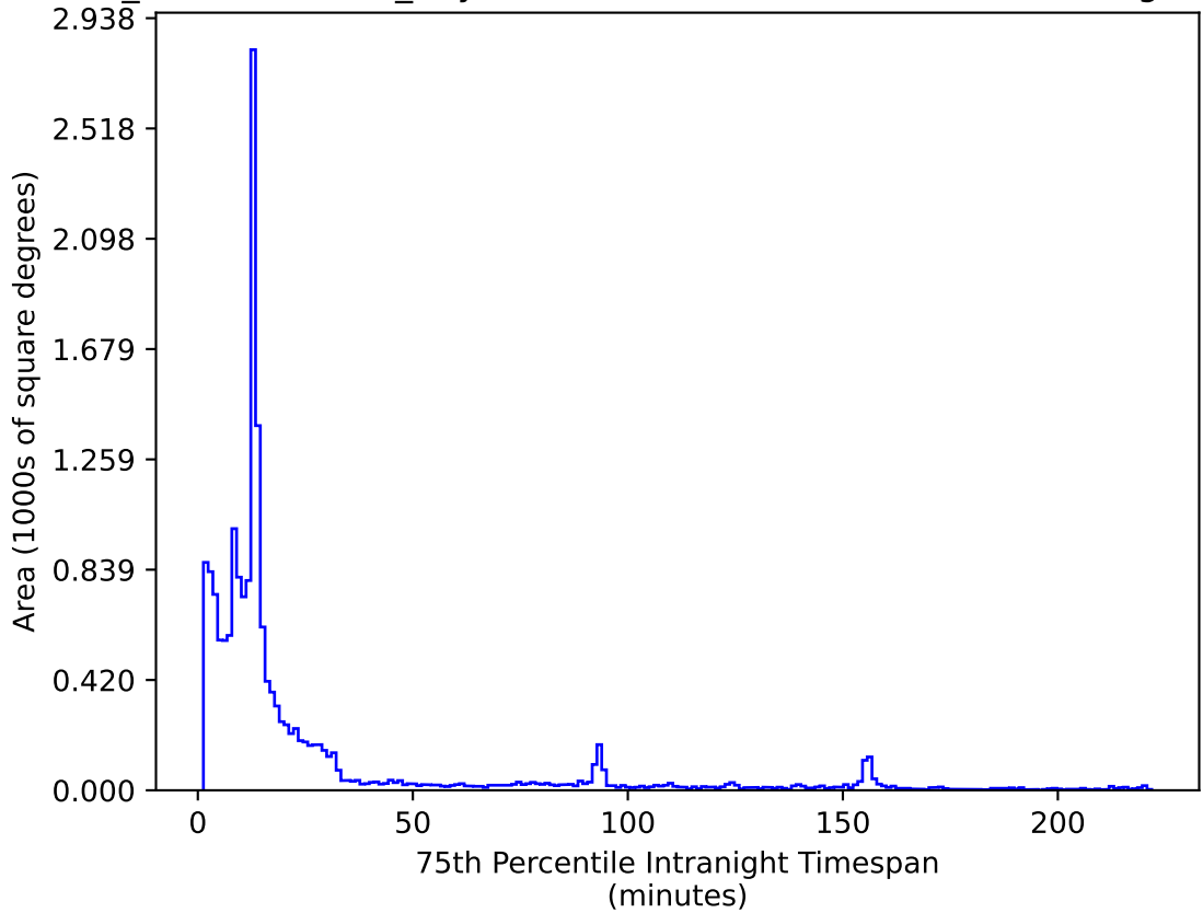
weather_cloudso31v3.4_10yrs WFD i band: 75th Percentile Intranight Timespan
