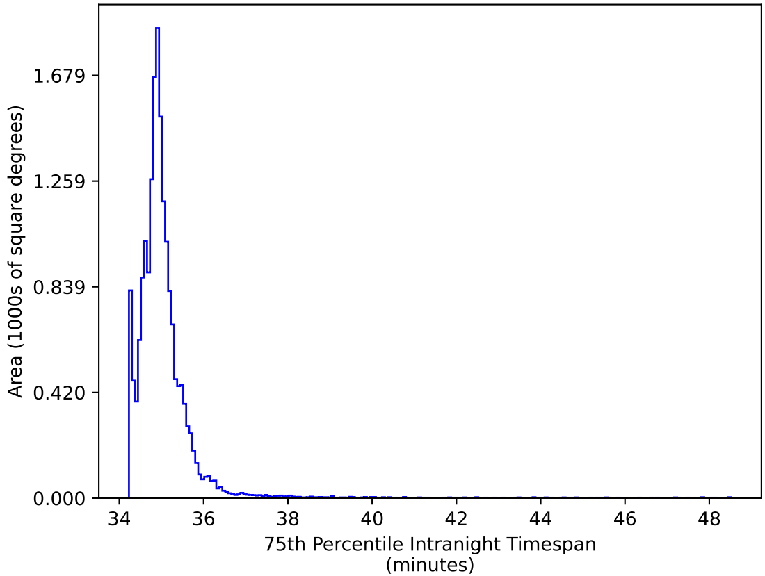
weather_cloudso31v3.4_10yrs WFD gr bands: 75th Percentile Intranight Timespan
