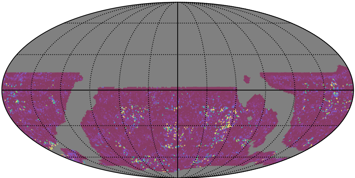
weather_cloudso31v3.4_10yrs WFD g band: 75th Percentile Intranight Timespan
