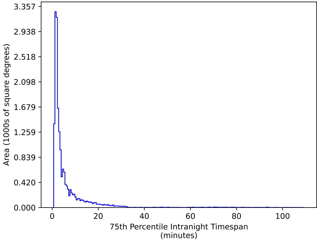
weather_cloudso31v3.4_10yrs WFD g band: 75th Percentile Intranight Timespan
