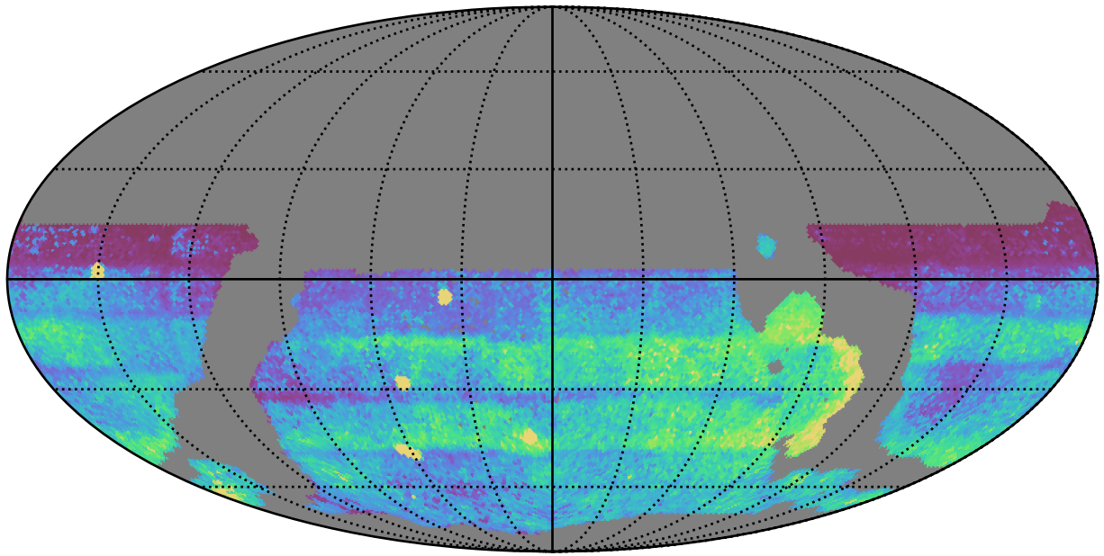
weather_cloudso31v3.4_10yrs WFD all bands: 75th Percentile Intranight Timespan
