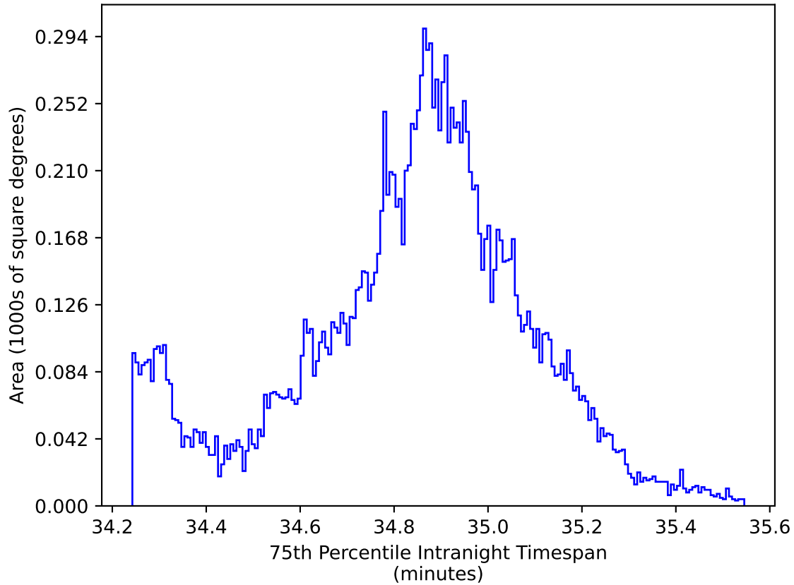
weather_cloudso31v3.4_10yrs WFD all bands: 75th Percentile Intranight Timespan
