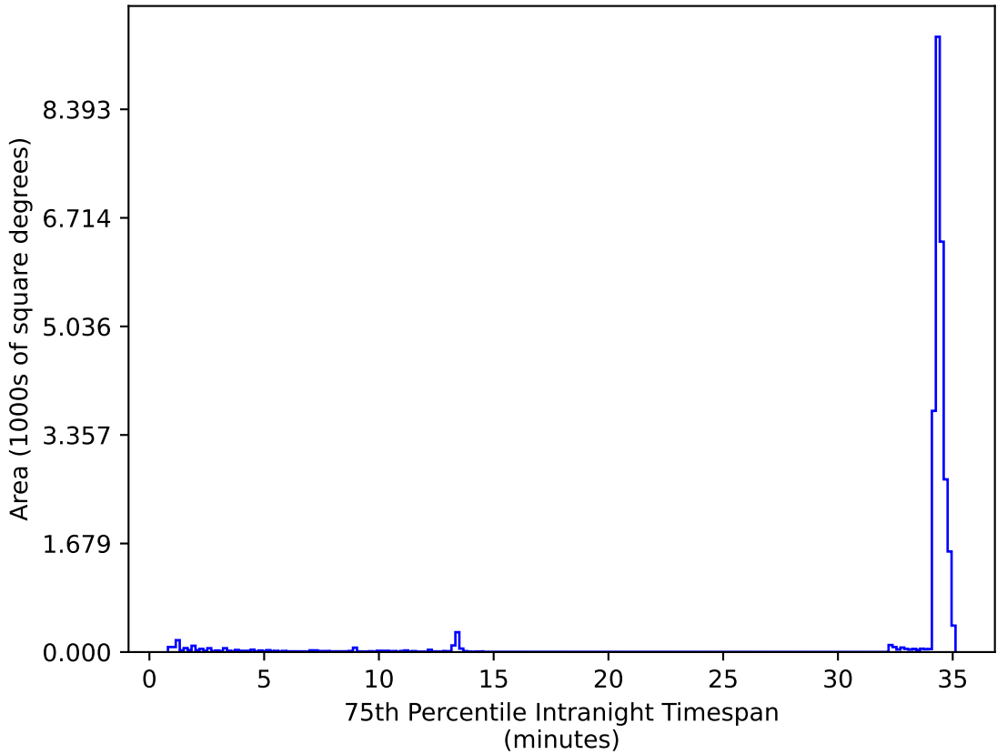
weather_cloudso31v3.4_10yrs All sky zy bands: 75th Percentile Intranight Timespan
