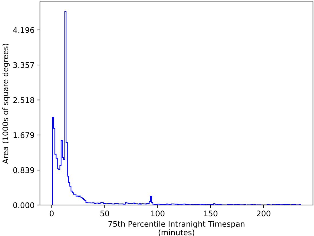
weather_cloudso31v3.4_10yrs All sky z band: 75th Percentile Intranight Timespan
