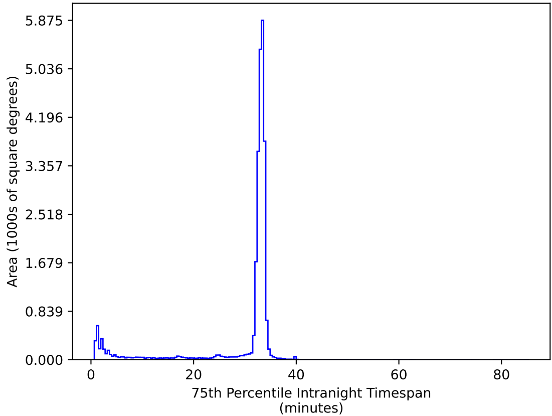
weather_cloudso31v3.4_10yrs All sky ug bands: 75th Percentile Intranight Timespan
