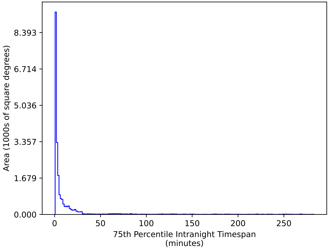
weather_cloudso31v3.4_10yrs All sky u band: 75th Percentile Intranight Timespan
