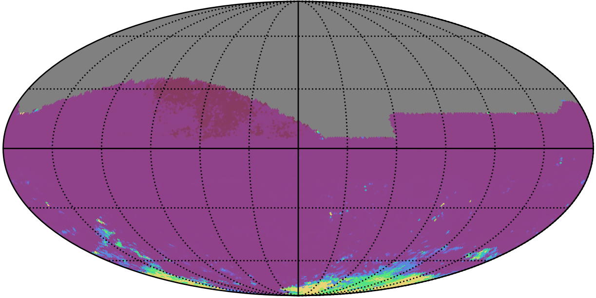
weather_cloudso31v3.4_10yrs All sky ri bands: 75th Percentile Intranight Timespan
