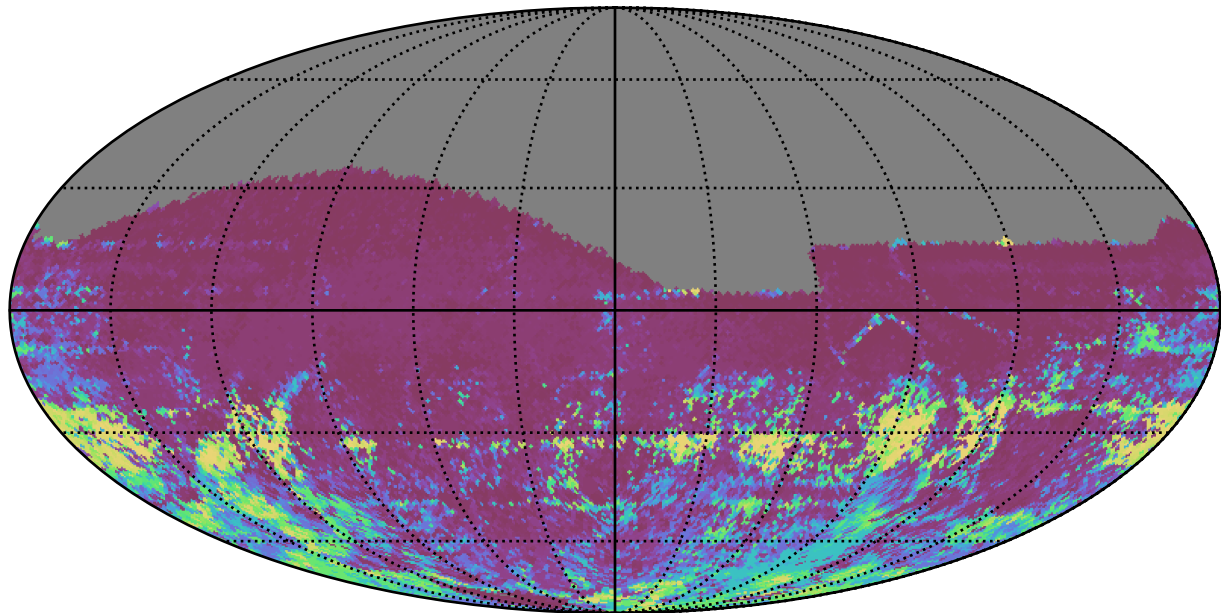
weather_cloudso31v3.4_10yrs All sky r band: 75th Percentile Intranight Timespan
