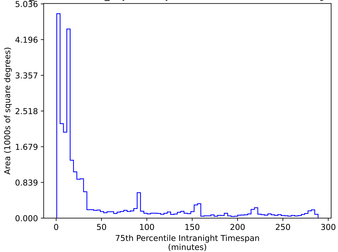
weather_cloudso31v3.4_10yrs All sky r band: 75th Percentile Intranight Timespan
