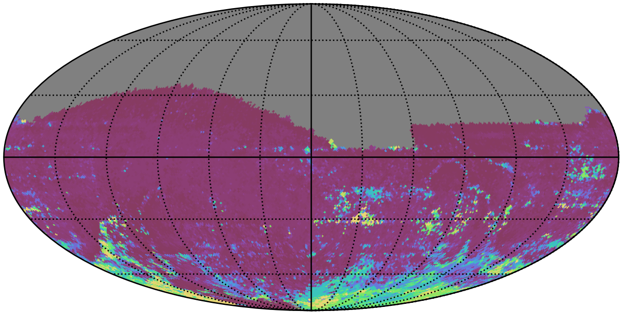
weather_cloudso31v3.4_10yrs All sky i band: 75th Percentile Intranight Timespan
