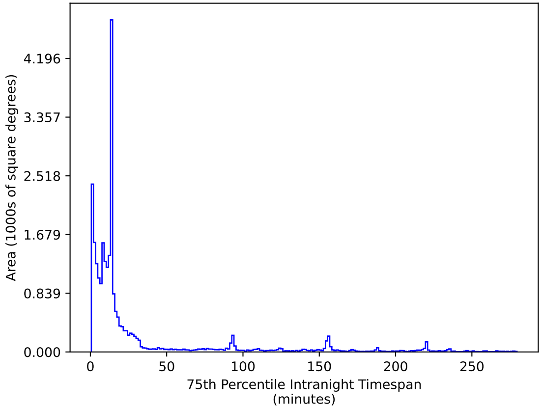
weather_cloudso31v3.4_10yrs All sky i band: 75th Percentile Intranight Timespan
