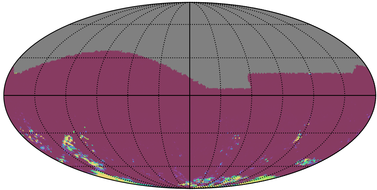
weather_cloudso31v3.4_10yrs All sky gr bands: 75th Percentile Intranight Timespan
