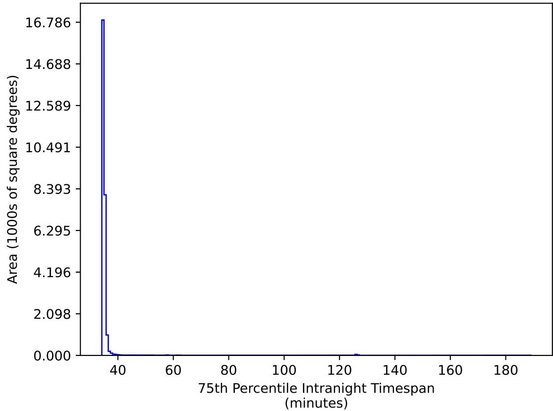
weather_cloudso31v3.4_10yrs All sky gr bands: 75th Percentile Intranight Timespan
