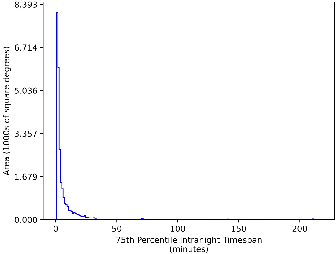
weather_cloudso31v3.4_10yrs All sky g band: 75th Percentile Intranight Timespan
